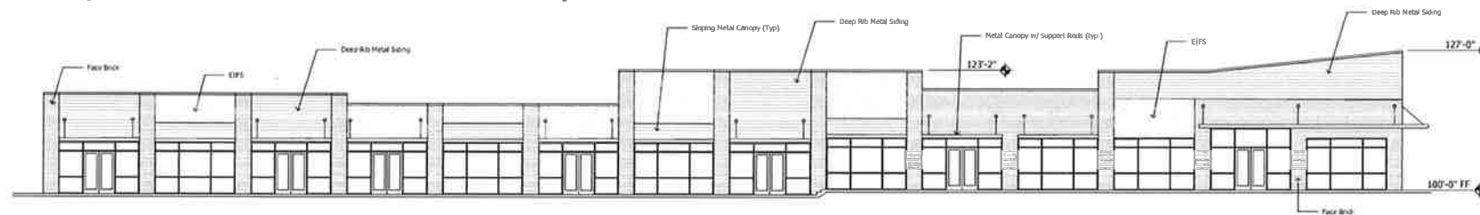
west elevation building B 3/32"=1'-0"
