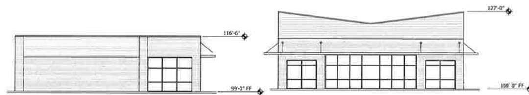
north elevation building B 3/32"=1'-0"
