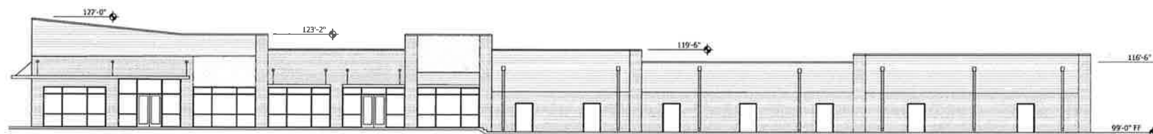
east elevation building B 3/32"=1'-0"
